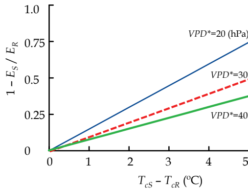
Fig. 3. The water stress index ( 1 - E_S / E_R ) as a function of the difference in the canopy temperature between rice and soybean ( T_{cS} - T_{cR} ) and the difference in the vapour pressure between the rice canopy and air ( VPD^* = e^*_{cR} - e_a ) (Eq. 12).
