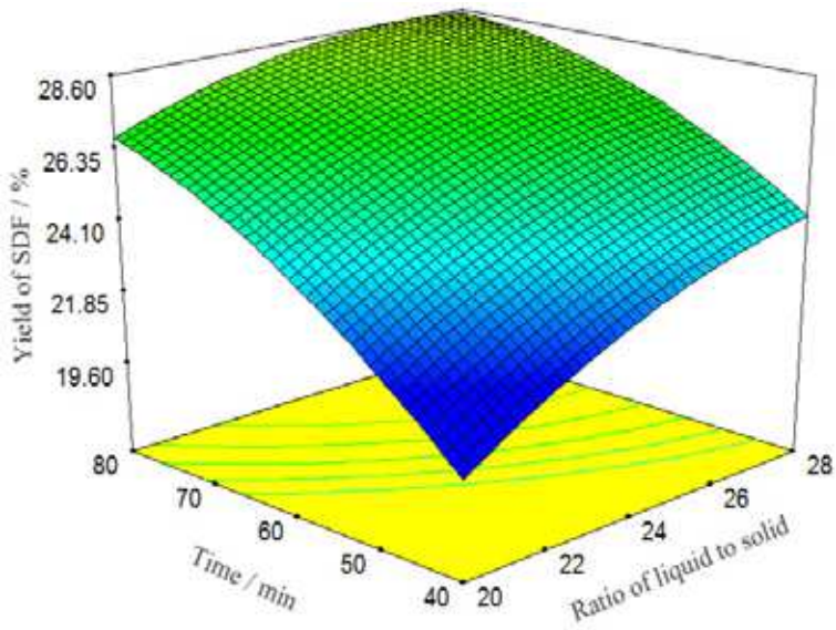
Fig. 3. Response surface for effects of ration of liquid to solid and time on the yield of SDF
