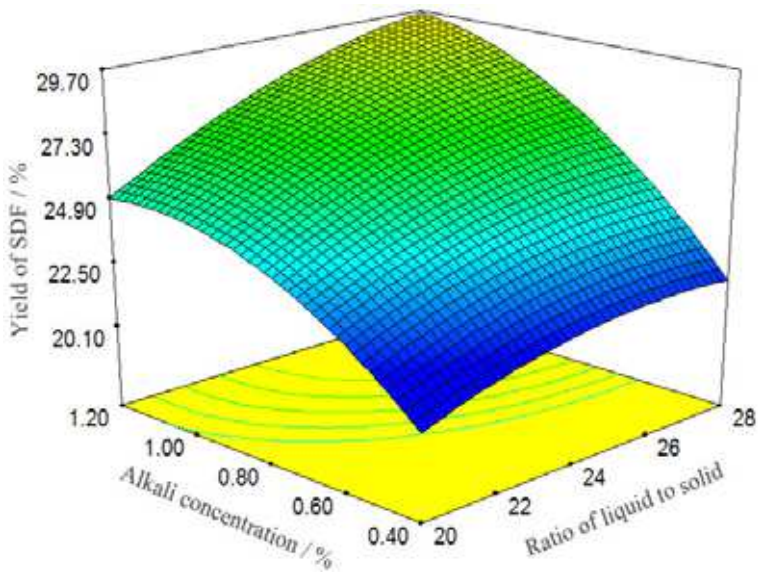
Fig. 4. Response surface for effects of ration of liquid to solid and alkali concentration on the yield of SDF
