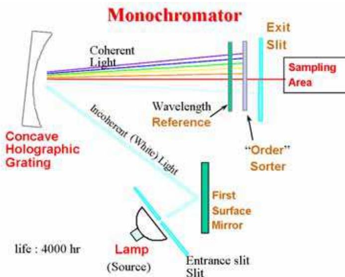
Fig. 2. General schematic of monochromator.
